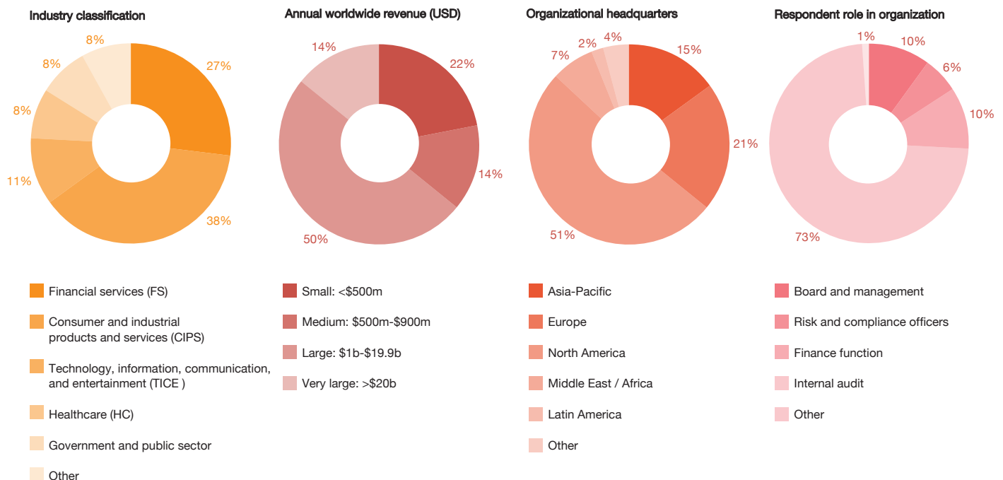
Figure 11: Respondent demographics
